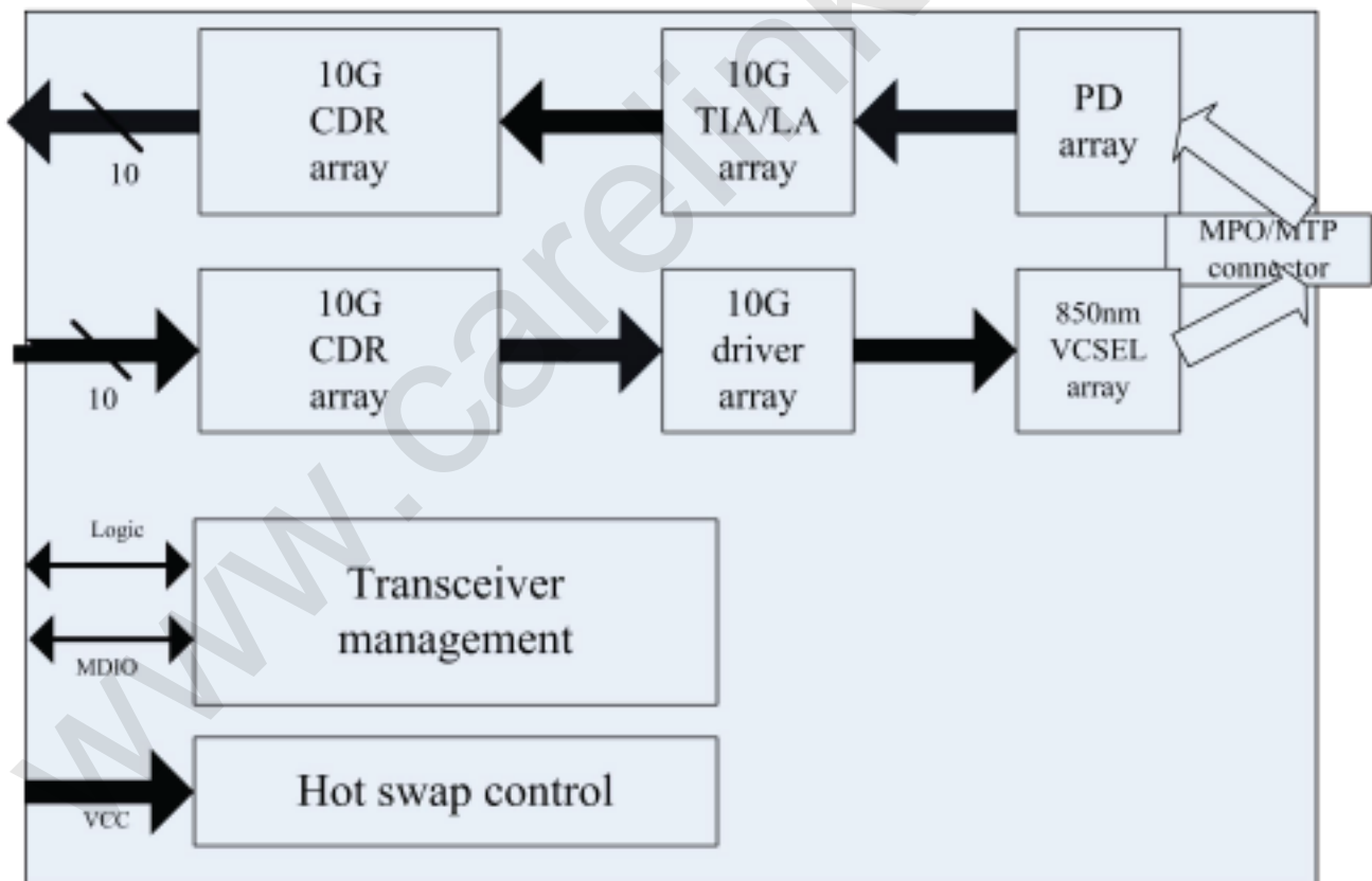
Module Block Diagram
