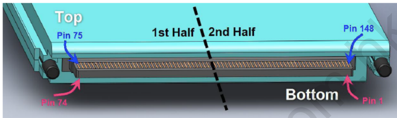
Pad Layout of the CFP module
