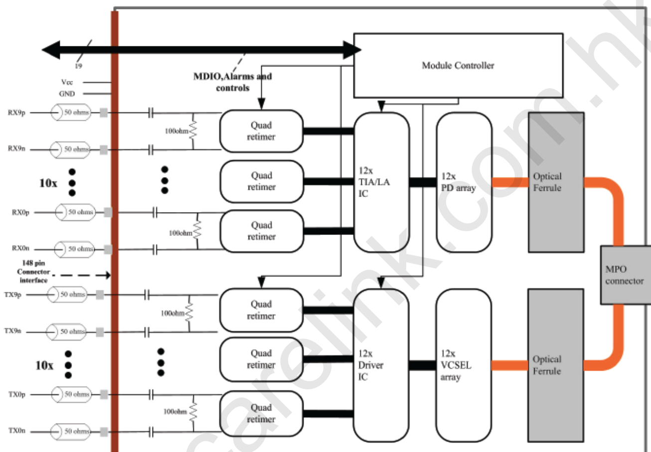
CFP module functional block diagram
